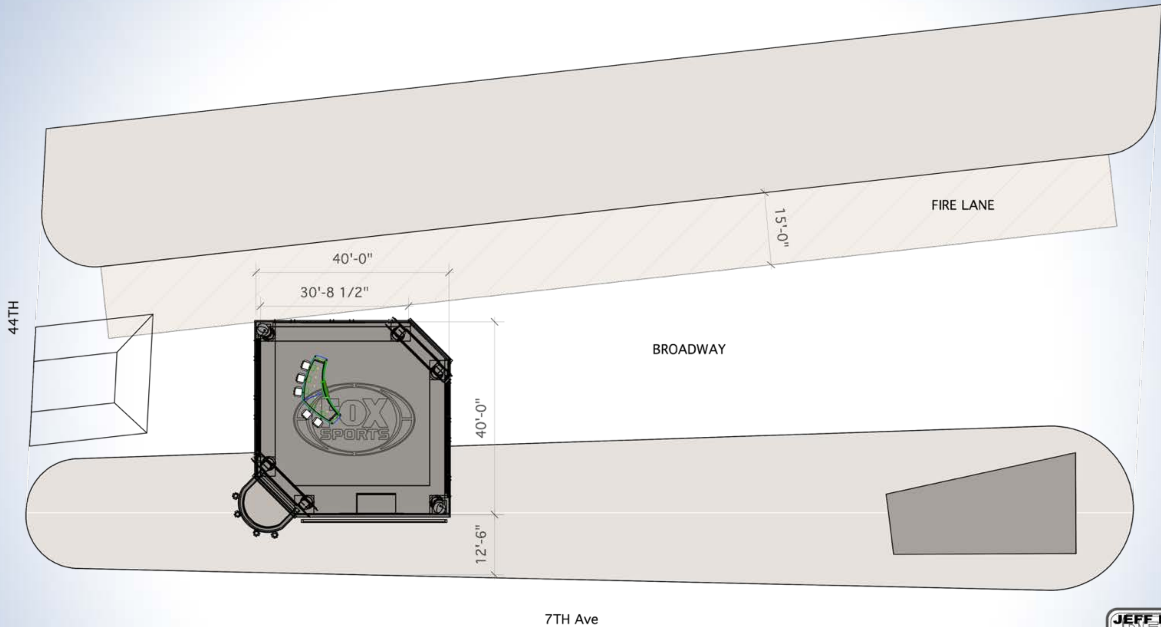
1 Fox Broadcast Tower NYC Plan Scale: 1/16" = 1'-0"
